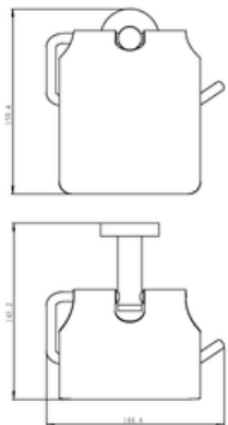
AVIV PH01 Paper Holder (Matt)
