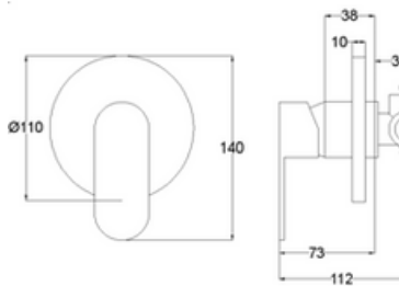
AVIV CSCYS SINGLE LEVEL CONCEALED MIXER STOPCOCK
