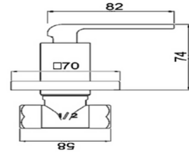
AVIV CSCSTF SINGLE LEVEL CONCEALED STOPCOCK
