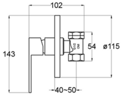
AVIV CSCSK SINGLE LEVEL CONCEALED STOPCOCK
