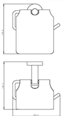
AVIV PH01-BK Paper Holder (Black)
